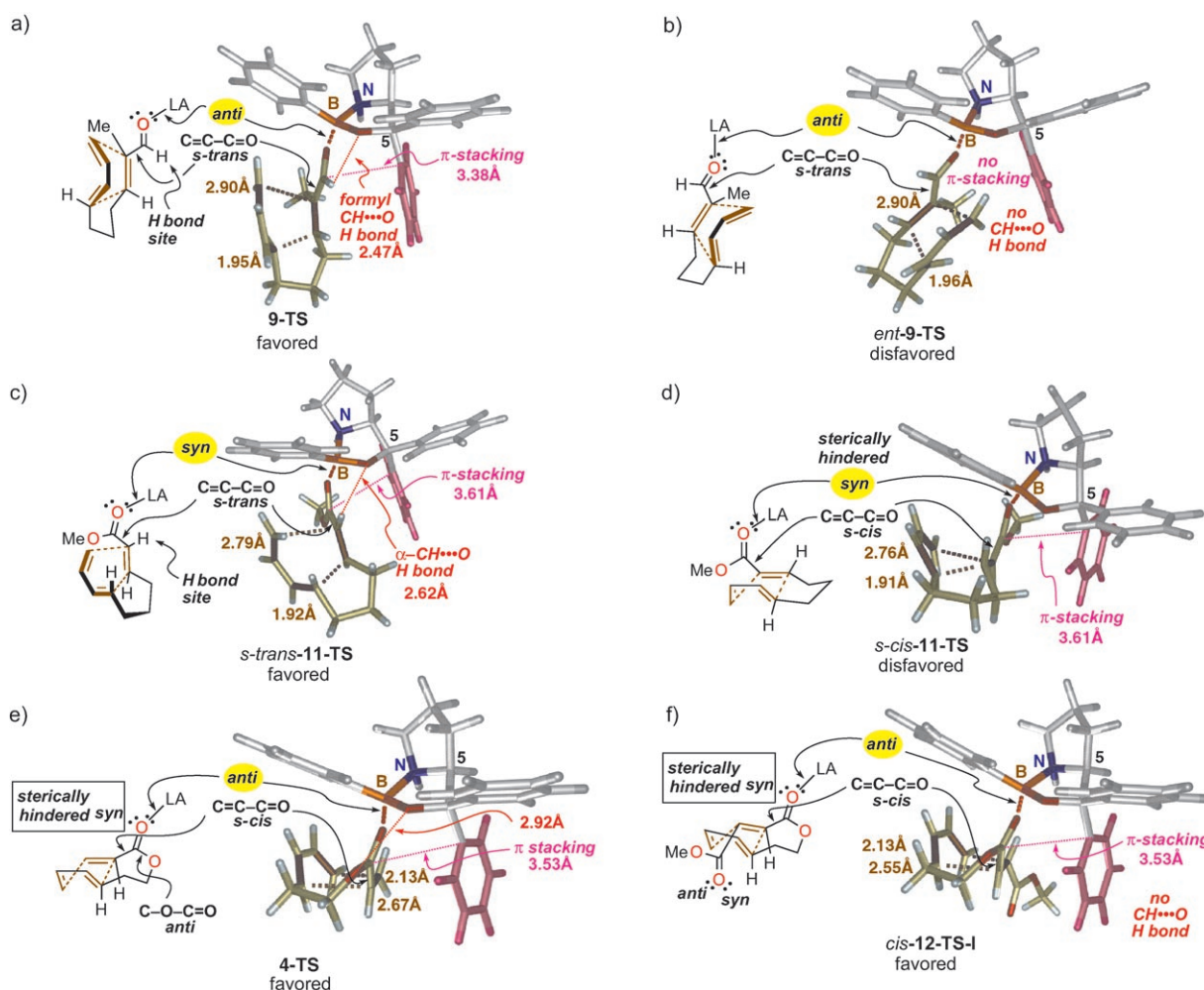
Figure 2. PCM B3LYP/6-31G(d) calculated transition-state structures for intramolecular Diels–Alder reactions catalyzed by oxazaborolidinium 1b ·H + . a) and b) TSs for 9 ; c) and d) TSs for 11 ; e) TSs for 4 ; f) TSs for 12 .
