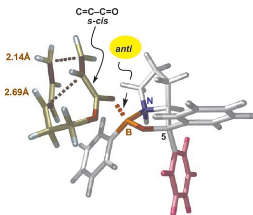
Figure 4. The lowest free energy TS for the DA reaction of 4 leading to formation of the minor enantiomer.
