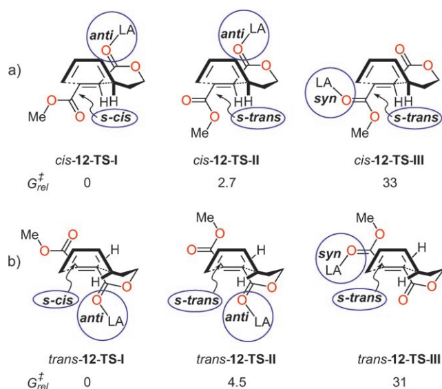
Figure 3. Relative free energies ( \text{kJ mol}^{-1} ) for selected a) cis -TSs and b) trans -TSs for fumarate 12 (LA = 1b ·H + ).
