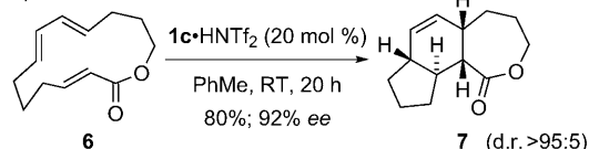
Scheme 2. DA reactions proceeding with enantioselectivities that vary relative to those predicted by the Corey O⋯HC hydrogen-bonding model. a) and b) are results from this work, and c) is a result from the work of Balskus and Jacobsen. [14]
