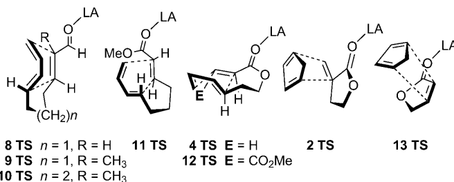
Figure 1. Schematic representation of the favored TS for each 1b ·H + -catalyzed DA reaction studied. The depicted diastereoselectivities ( cis or trans for triene precursors and endo or exo for dienophiles) and \pi -enantiofacial selectivities are those favored experimentally (LA = 1b ·H + ).
