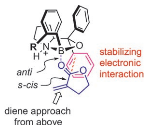
Figure 5. The new pre-transition-state model explaining the unexpected enantioselectivity with s-cis \text{C}=\text{C}-\text{C}=\text{O} , ester-activated dienophiles.
