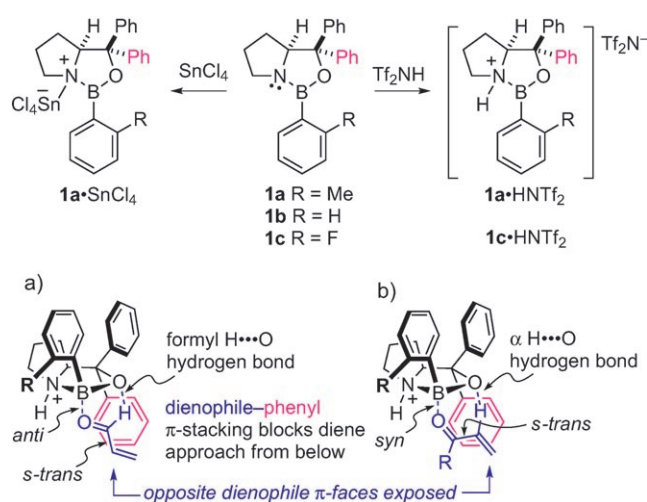
Scheme 1. Corey's oxazaborolidinium catalyst and pre-transition-state models (i.e. diene absent). a) Proposed mode of complexation for aldehydes. b) Proposed mode of complexation for ketones, esters, and acids.
